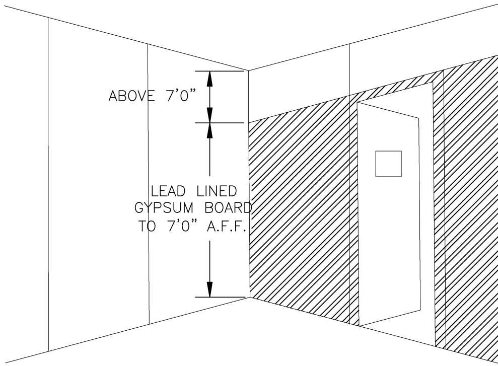
LEAD HEIGHT DETAIL NOT TO SCALE
