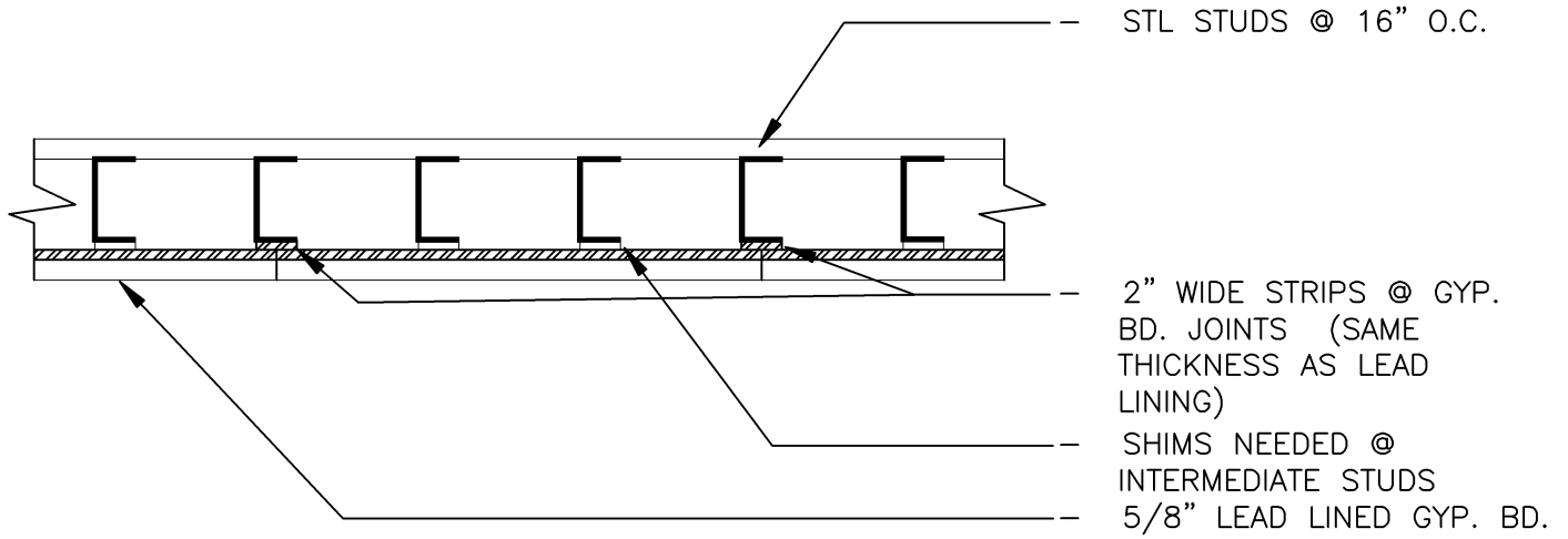
WALL DETAIL NOT TO SCALE
