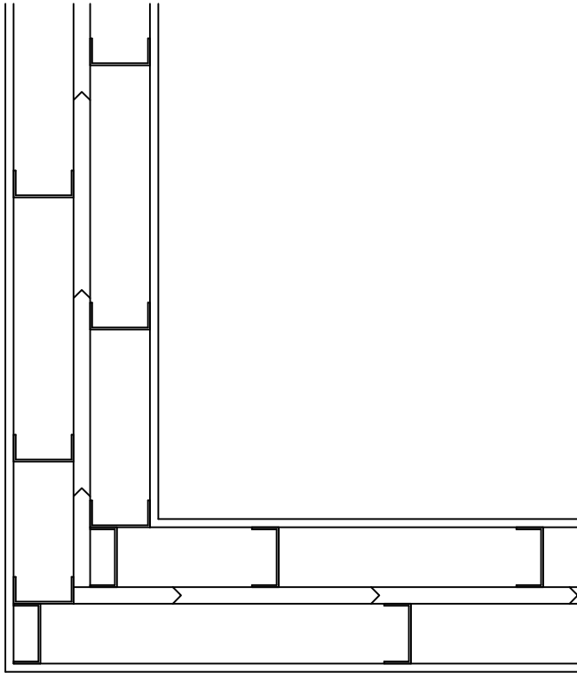
CORNER DETAIL
